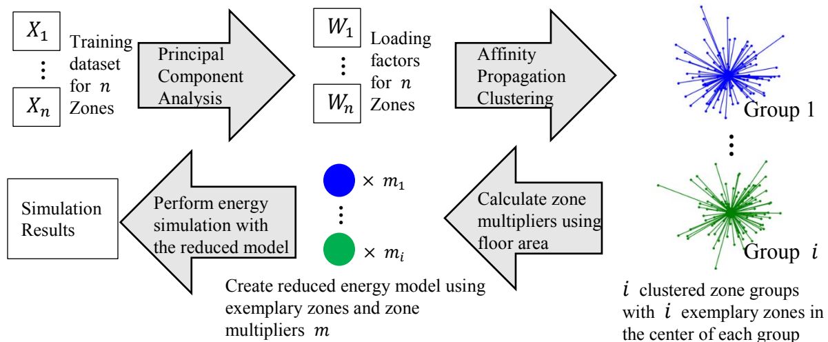
Figure 1. Procedures of the proposed model reduction method
