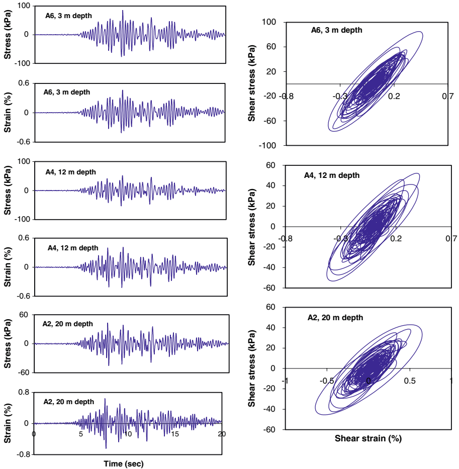
Fig. 4 Shear stress–strain histories at different depths during WCM event, model RG-01
