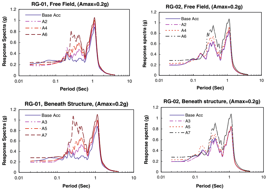
Fig. 8 Response spectra with peak base acceleration of 0.2
