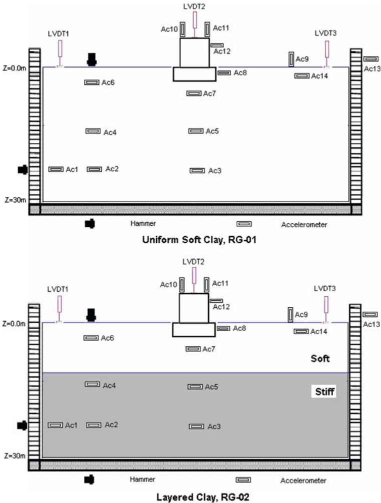
Fig. 1 Centrifuge model con guration in prototype scale
