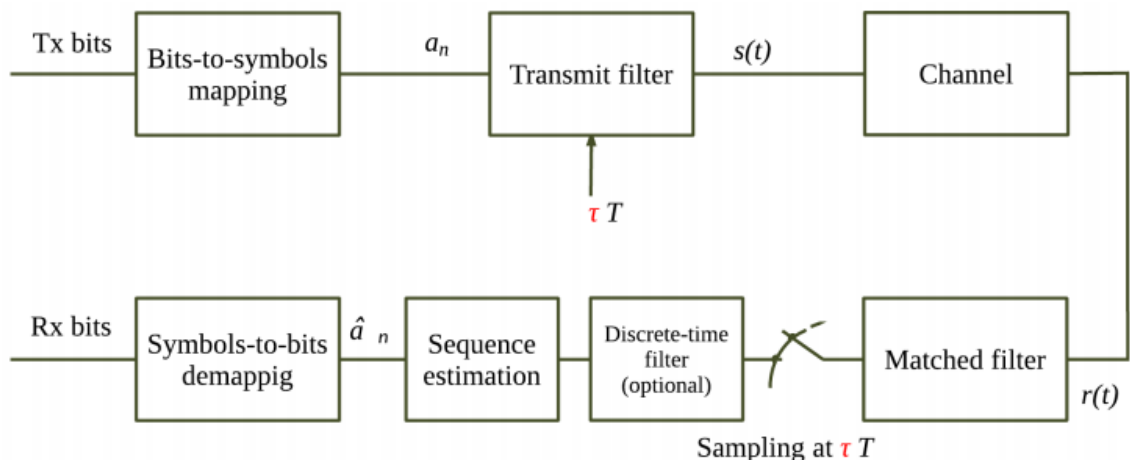
Fig. 1: Block diagram of FTN system
