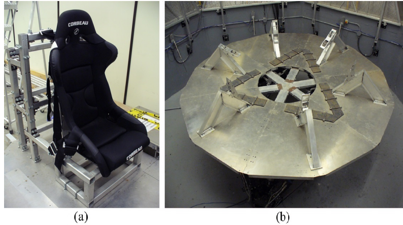
Fig. 5: (a) Floor structure and pilot support system; (b) interface platform which supports the sphere is attached to the Moog hexapod.
