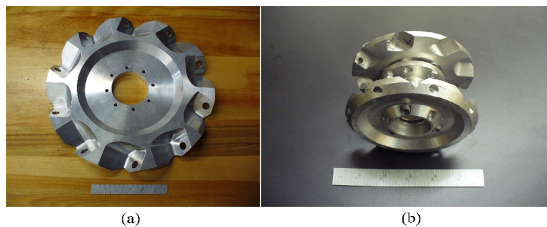
Fig. 7: (a) Atlas active wheel hub; (b) Atlas passive wheel hub assembly.
