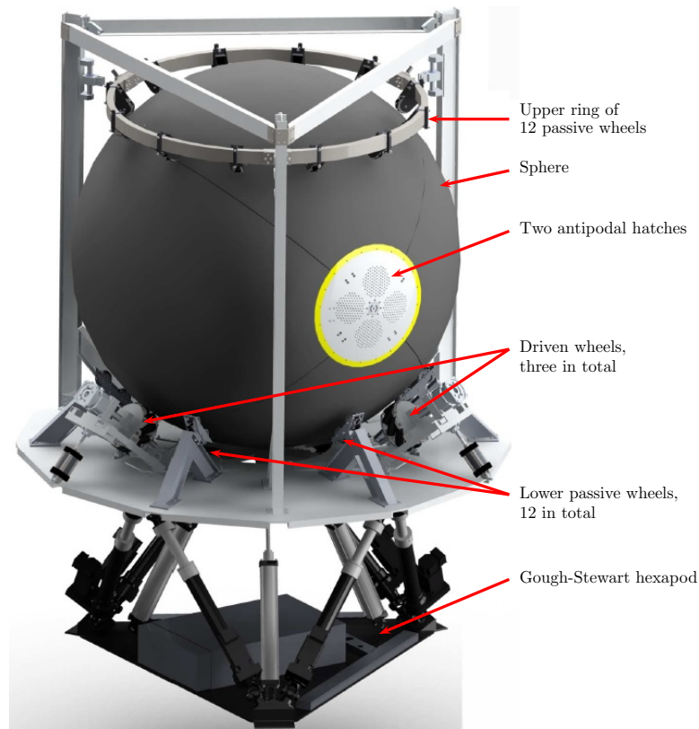
Fig. 1: A 3D rendering of the Atlas simulator.
