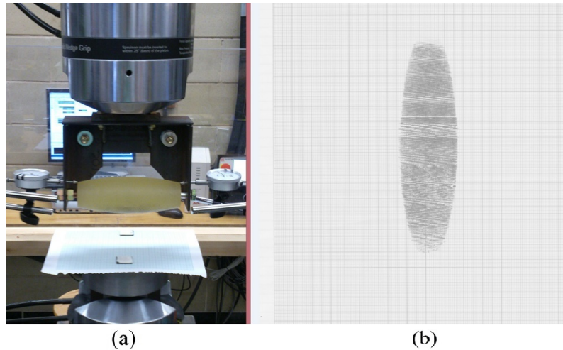
Fig. 8: (a) MTS press test frame with sample roller inserted; (b) resulting ink blot after compression testing a durometer 55A urethane to 1300 lbf.
