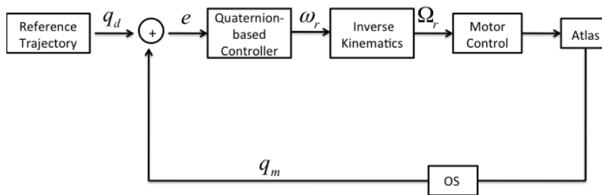
Fig. 9: Angular motion feedback control loop.
