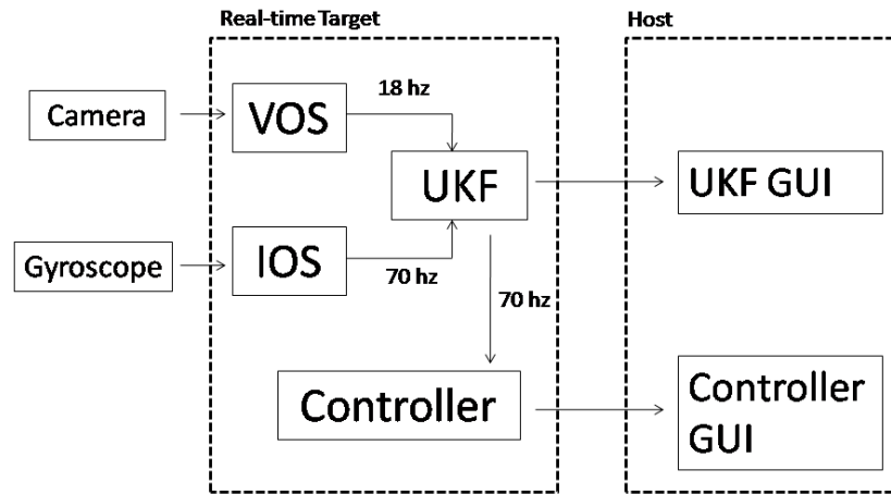
Fig. 10: Orientation data fusion algorithm.
