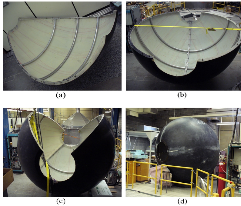
Fig. 3: Assembling the four sphere panels.
