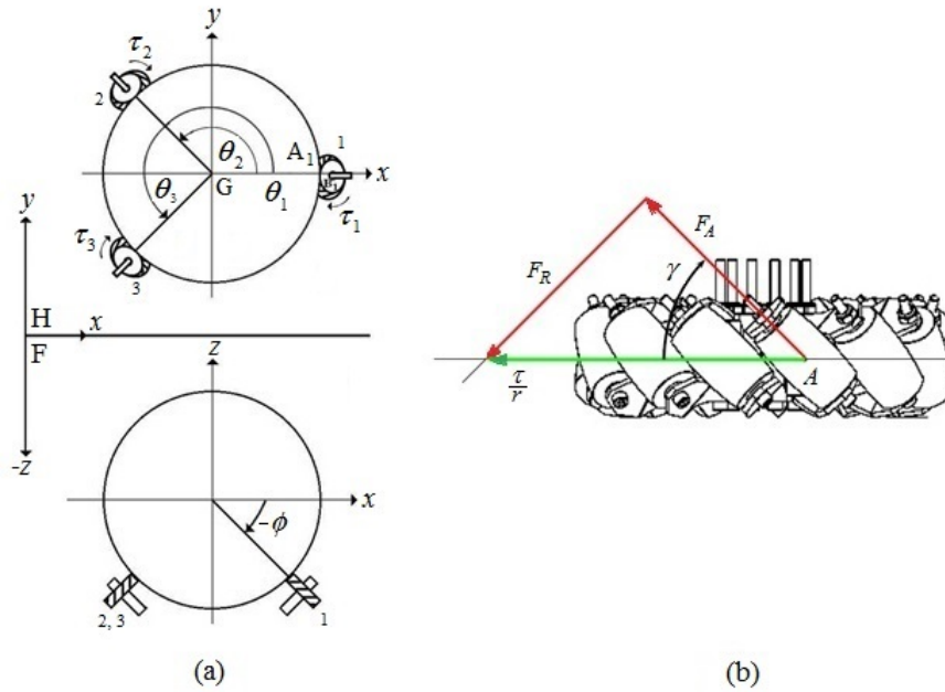
Fig. 12: (a) Mecanum wheel position around sphere; (b) roller angles around Mecanum wheel.
