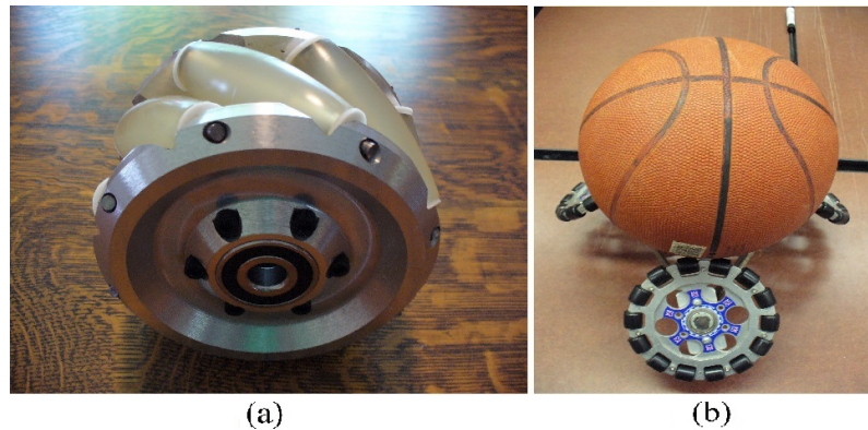
Fig. 6: (a) CUSP Mecanum wheel design; (b) omniwheel proof of concept model.
