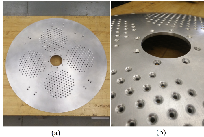
Fig. 4: (a) Top down view of one Atlas hatch; (b) detailed view of contoured ventilation holes.
