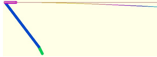
Figure 3: Deformed beam shape predicted by ADAMS simulation
