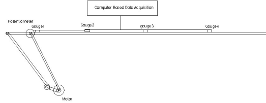
Figure 2: Schematic illustration of mechanism configuration and strain gauge attachment points
