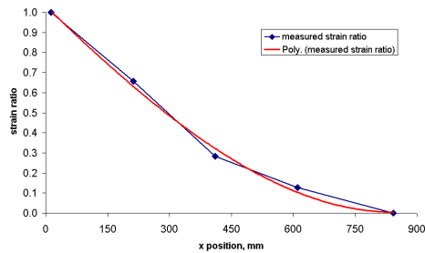
Figure 7: Strain ratio as a function of position along the beam
