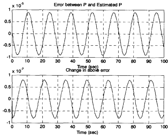
Fig. 41 e_{p_k} and \dot{e}_{p_k} [Sasiadek, J.Z., and Khe, J., (2001)]
