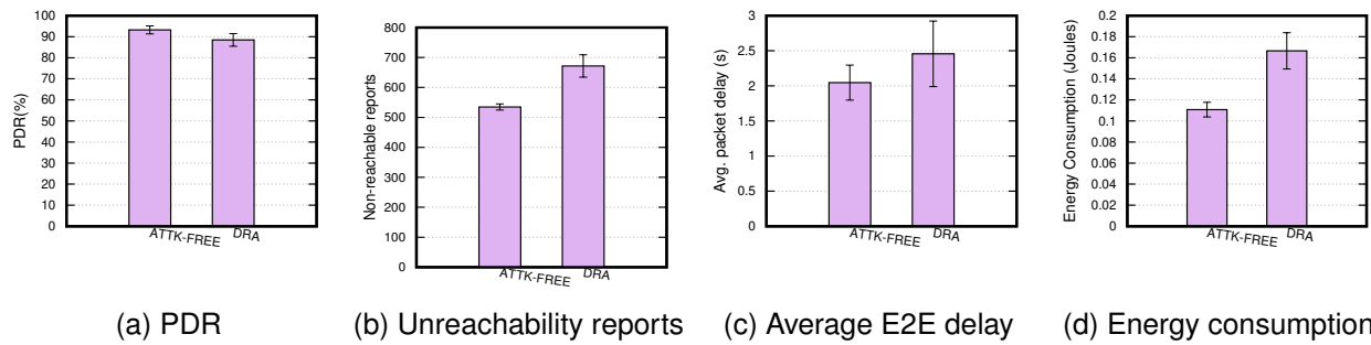
Fig. 6. The impact of the DRA on the 6TiSCH network performance and energy consumption
