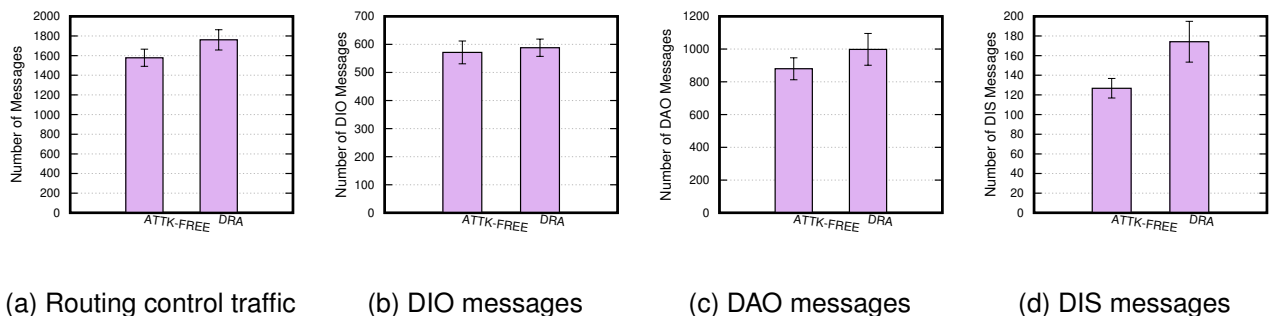
Fig. 3. The impact of the DRA on the RPL control messages transmission
