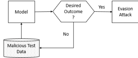
Fig. 4. Evasion Attack
