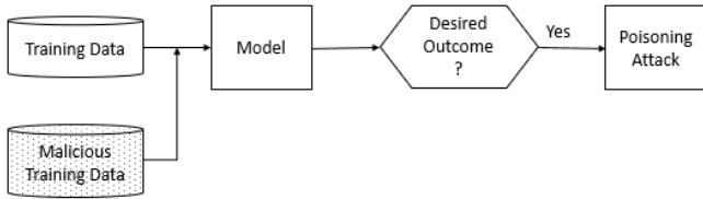
Fig. 5. Poisoning Attack
