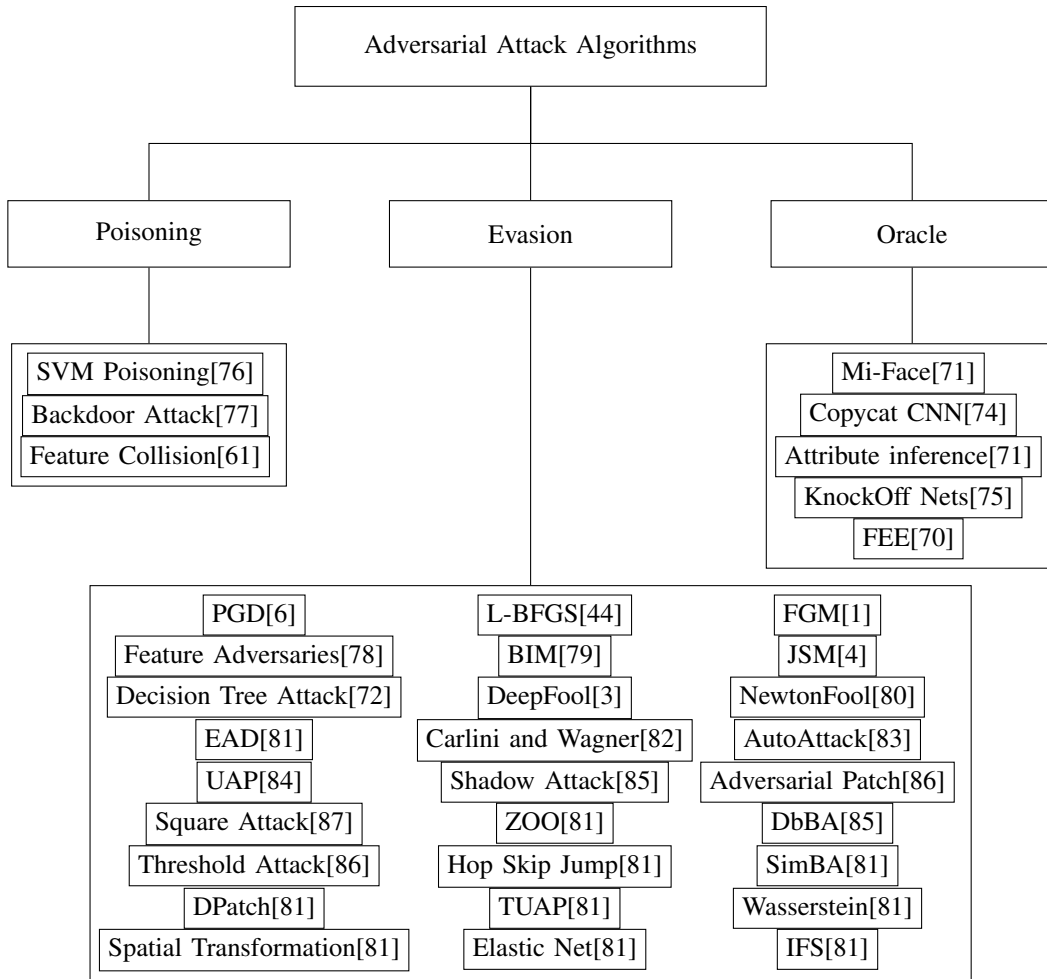
Fig. 6. Adversarial Attack Algorithms
