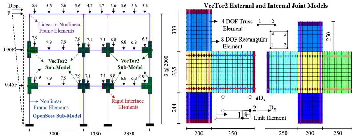
Fig. 6. Multi-platform model of RC frame with eight joints modelled with VecTor2 (dimensions in mm & forces in kN, 1 mm = 0.04 in., 1 kN = 0.225 kip).
