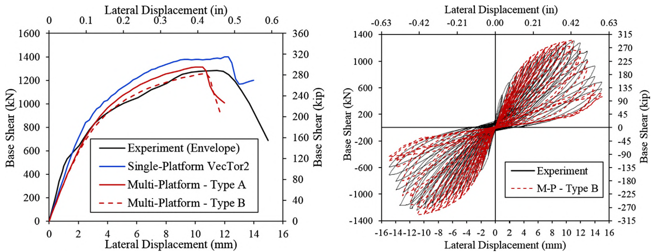
Fig. 4. Load-deflection responses of shear wall for push-over and reversed cyclic analyses.
