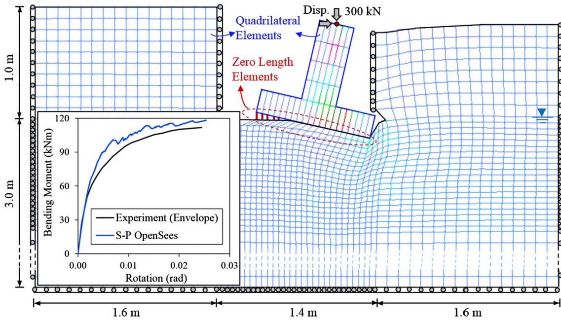
Fig. 10. OpenSees model and moment-rotation responses of soil-foundation system tested by Negro et al. [38] (dimensions in m & forces in kN, 1 m = 39.4 in., 1 kN = 0.225 kip).
