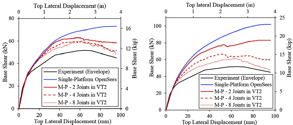
Fig. 7. Load-deflection responses of frame for push-over analyses of Type A models (left) and Type B models (right).
