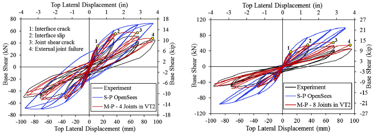
Fig. 8. Load-deflection responses of frame for reversed cyclic analyses of Type A models (left) and Type B models (right).
