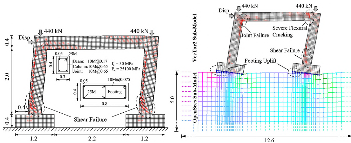
Fig. 11. Damage modes for single-platform VecTor2 analysis (left) and multi-platform analysis (right) (dimensions in m & forces in kN, 1 m = 39.4 in., 1 kN = 0.225 kip).
