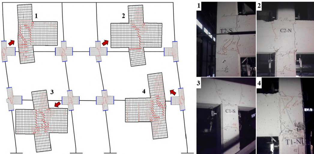
Fig. 9. Computed and experimentally reported crack patterns for RC frame.
