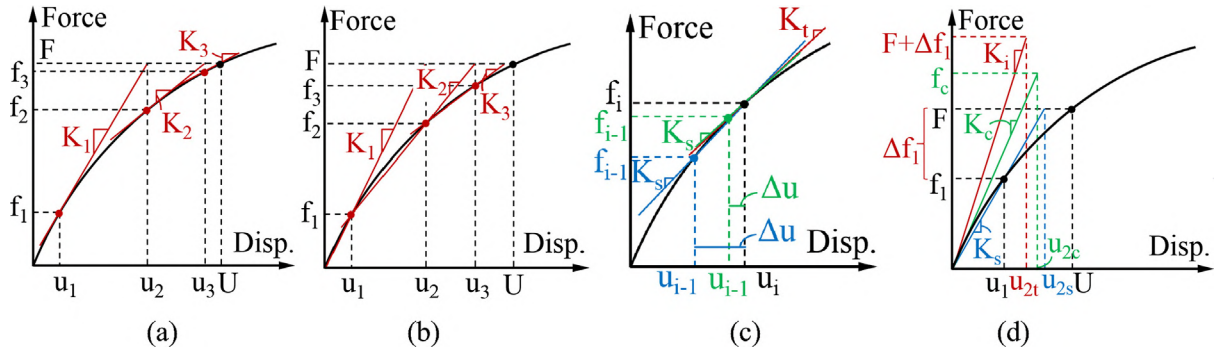
Fig. 1. (a) incremental tangent-based method; (b) incremental secant-based method; (c) approximation of secant method with tangent method; (d) combination of total solution methods.
