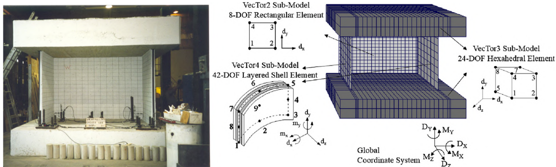
Fig. 3. Shear wall test specimen [36] (left) and Type B multi-platform FE model (right).
