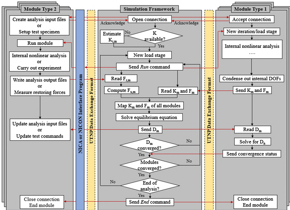
Fig. 2. Algorithm of the proposed multi-platform framework.
