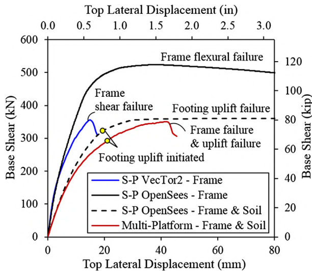
Fig. 12. Load-deflection responses of soil-structure system for different modelling approaches.
