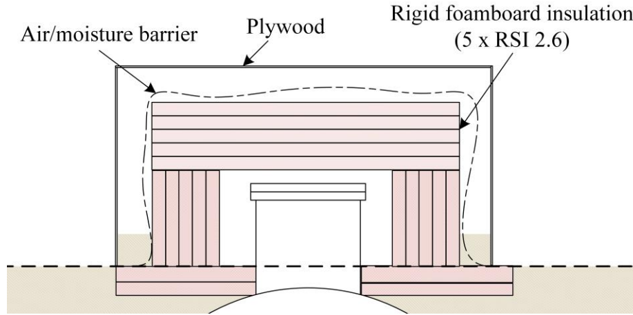
Fig. 4: Insulation of the STES access hatch
