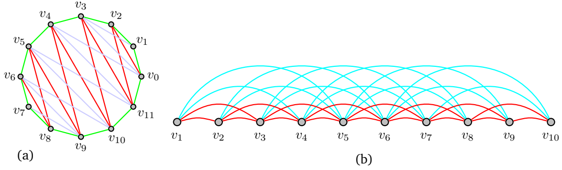
Figure 3: Edge-maximal layouts: (a) 2-stack, (b) 2-queue.
