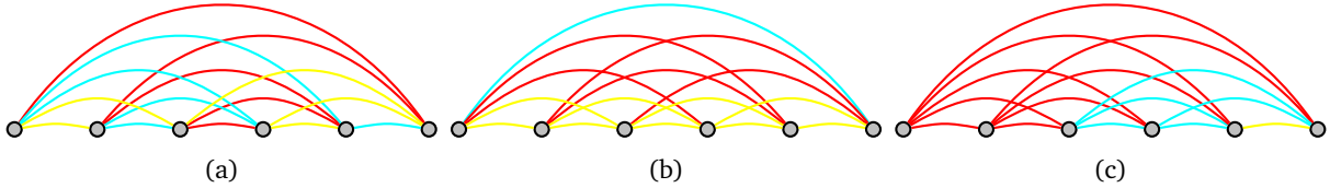
Figure 1: Layouts of K_6 : (a) 3-stack, (b) 3-queue, (c) 3-arch.
