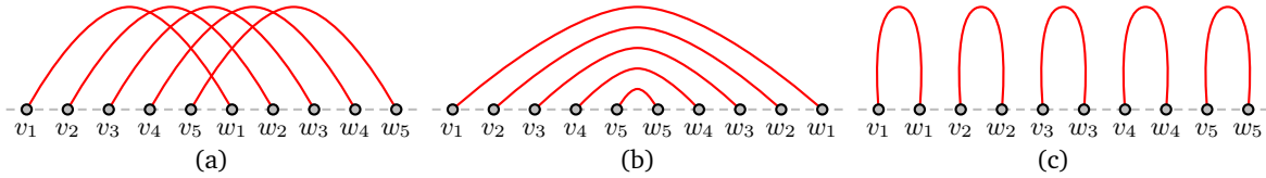
Figure 2: (a) 5-edge twist, (b) 5-edge rainbow, (c) 5-edge necklace.
