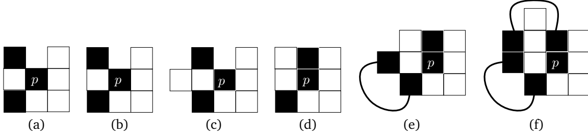
Figure 12: Illustrating Case 2 in the proof of Lemma 4.
