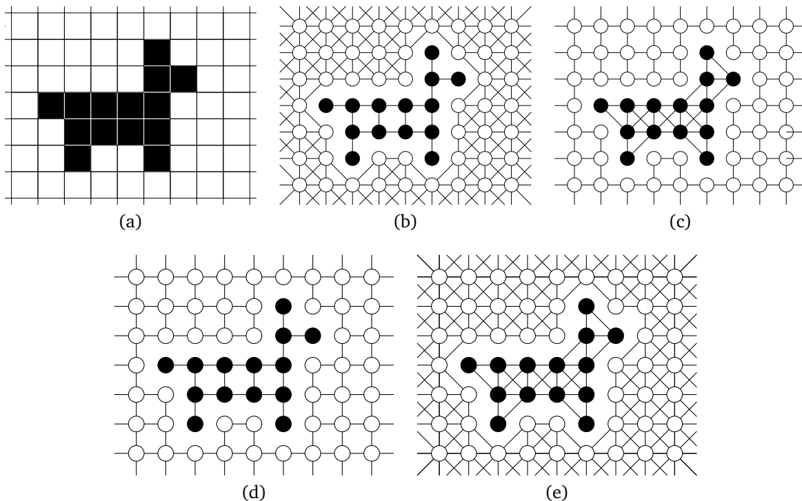
Figure 1: (a) a binary image I , (b) the graphs B_4(I) and W_8(I) , (c) the graphs B_8(I) and W_4(I) , (d) the graphs B_4(I) and W_4(I) , and (e) the graphs B_8(I) and W_8(I) .
