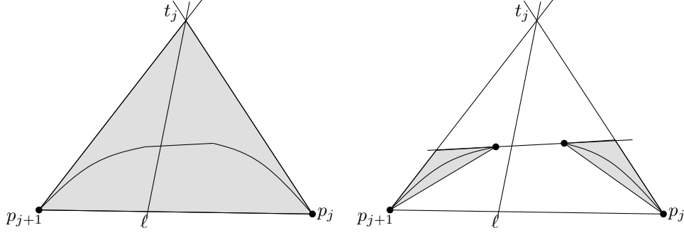
Figure 4: The data structure can be realized using only lines through the vertices of P .
