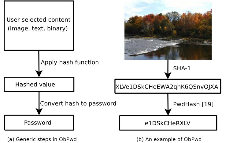
Figure 1: ObPwd steps with an example
