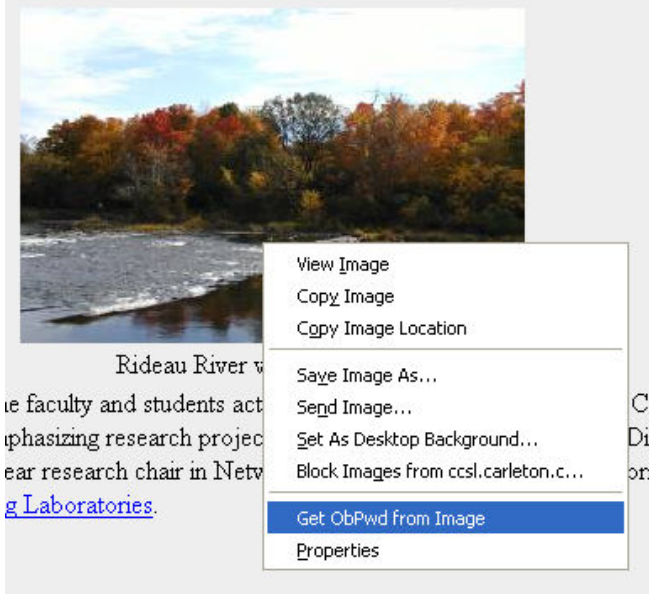
Figure 2: ObPwD extension menu in Firefox
