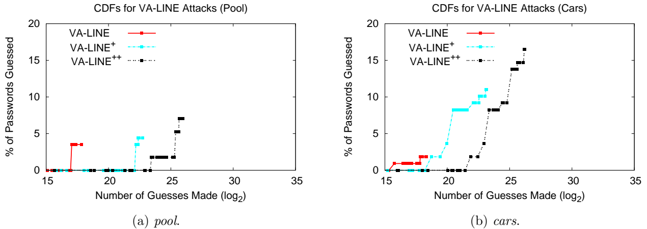
Figure 9: VA-LINE CDFs.
