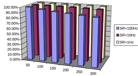
Fig. 11. LoCoM's throughput
