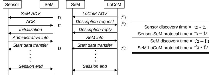
Fig. 4. Simplified Sensor-SeM-LoCoM protocol
