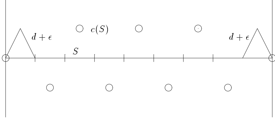
Figure 5: Companion points in the \epsilon -envelope. The figure depicts the sector assigned to e and the chain corresponding to e .
