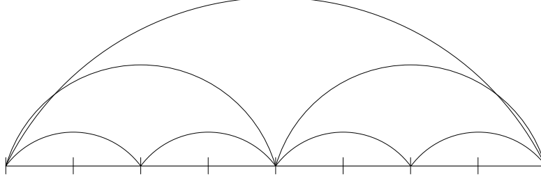
Figure 2: Tree-layout on a chain.
