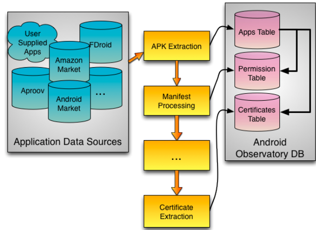
Figure 5: Block diagram of Observatory import process.
