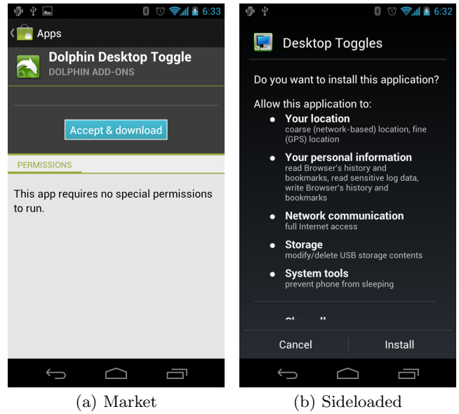
Figure 2: Screenshots of permissions requested by installing the Desktop Toggle browser extension via the Google Play Store and when side-loaded. In both cases, the Dolphin Browser had been previously installed.
