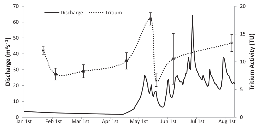
Figure 8. Measured tritium activity (expressed as TU) and total river discharge in the NKR, 2014.
